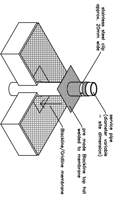
STANDARD TOP HAT TO SERVICE PIPE DETAIL
